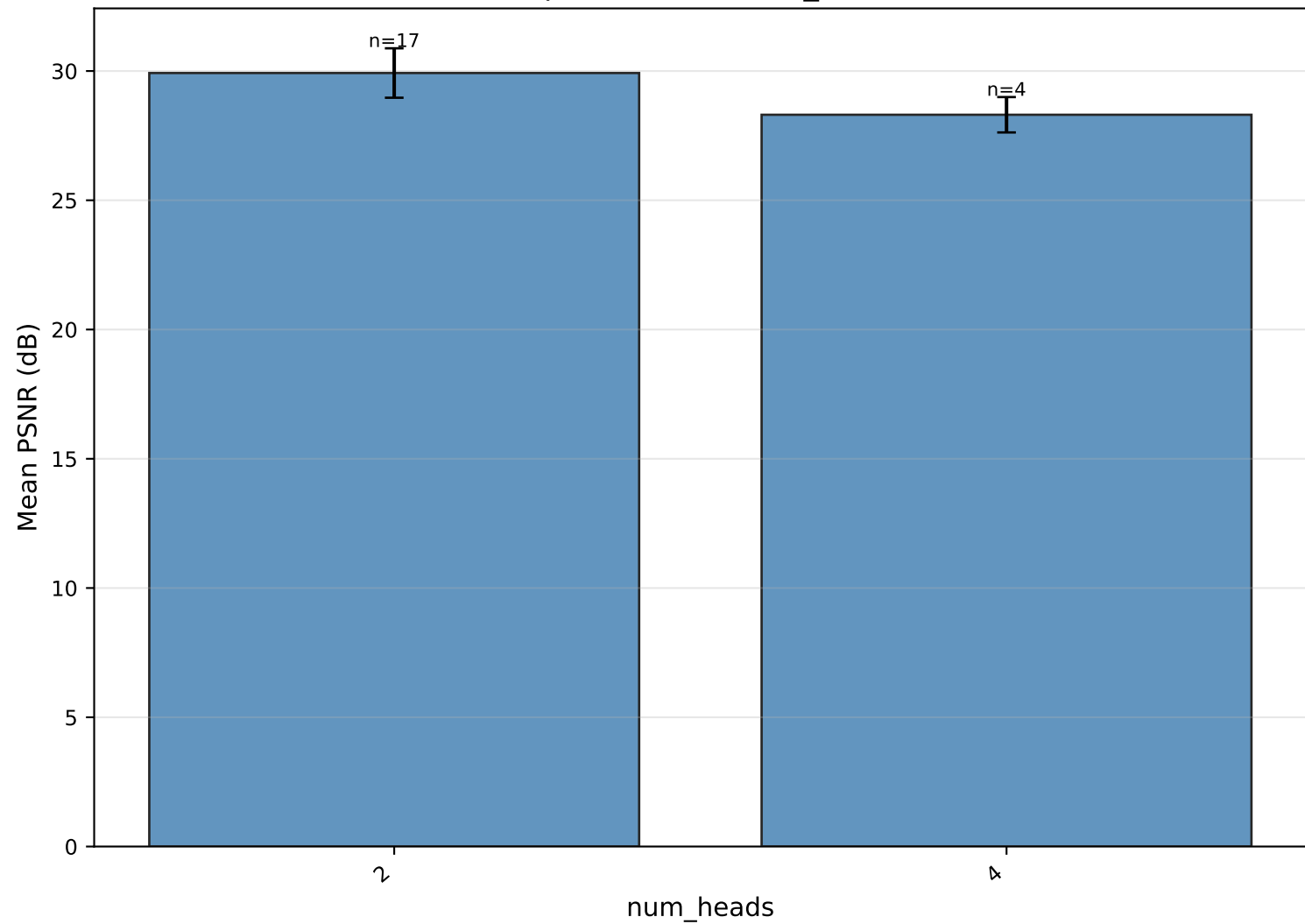
Mean PSNR per value of num_heads — ELAN
